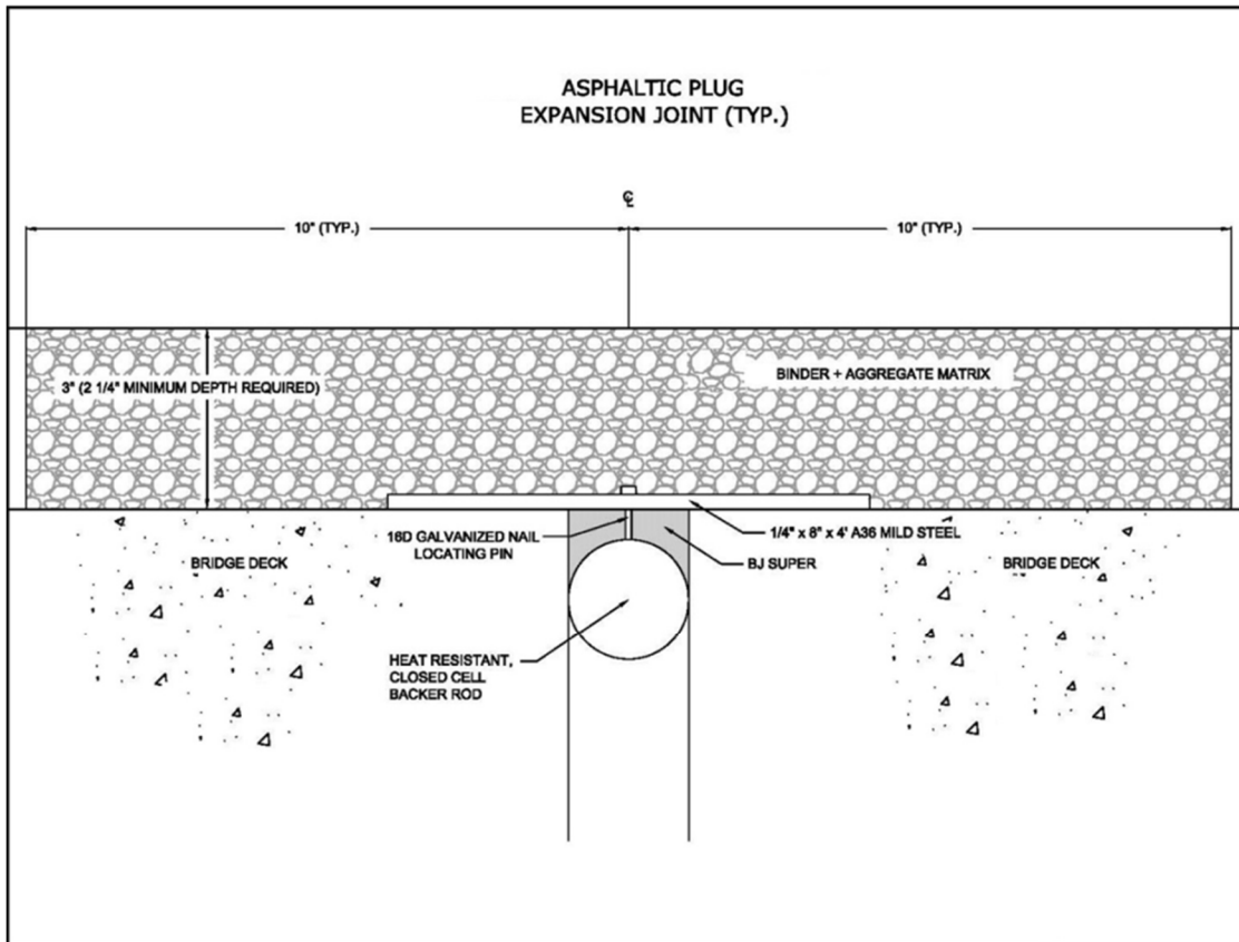
Asphaltic Plug Expansion
